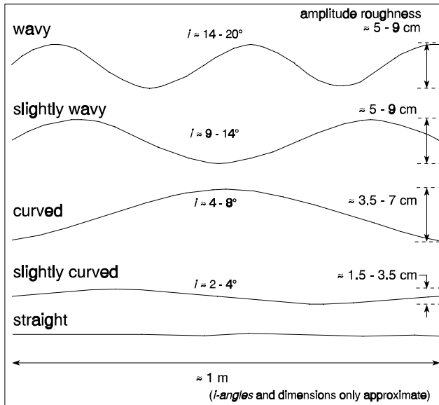
Fig. 3. Large scale roughness profiles.
