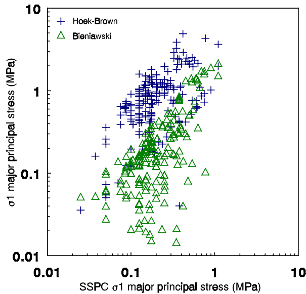
Fig. 5. Comparison of major effective principal stress values.
