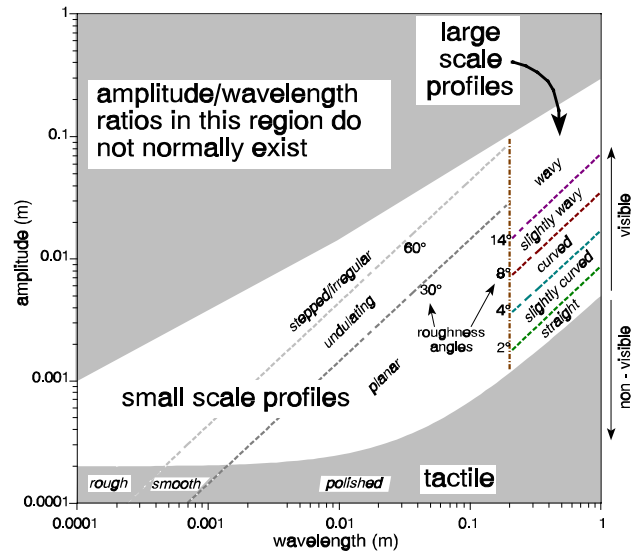
For small amplitudes and wavelengths the roughness is of a triangular/sawtooth form whereas with larger amplitudes and wavelengths the roughness changes to a more sinusoidal form. Lustre is not included in the boundary non-visible to visible roughness. The boundaries in the graph are dashed as these are not exact.
