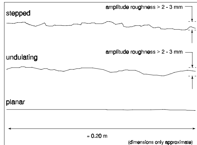
Fig. 4. Small scale roughness profiles.
