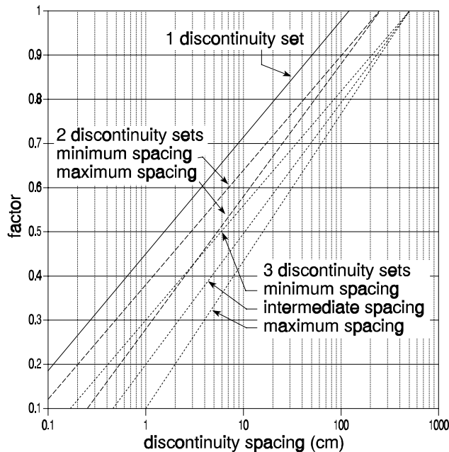
Fig. 1. Discontinuity spacing factors (after Taylor, 1980).
